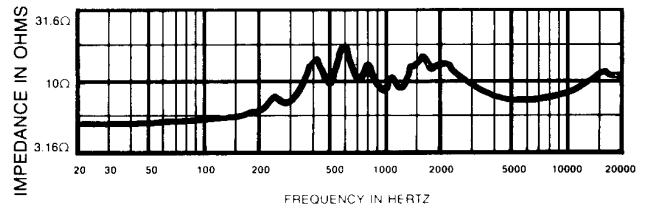
FIGURE 7 Impedance Response — HP9040 Horn 8-Ohm Driver
