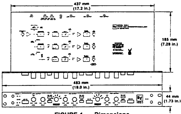
FIGURE 1 — Dimensions
