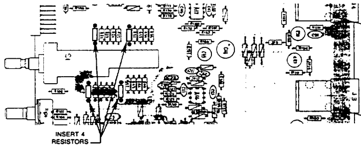
FIGURE 8 — Crossover-Frequency Modification
