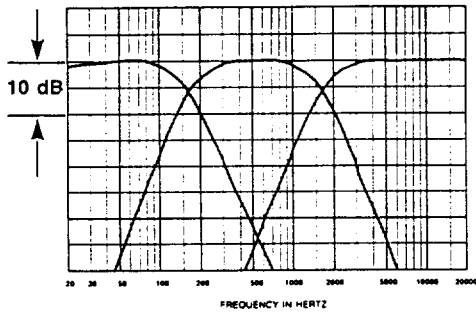
FIGURE 3 — Typical Crossover Curve
