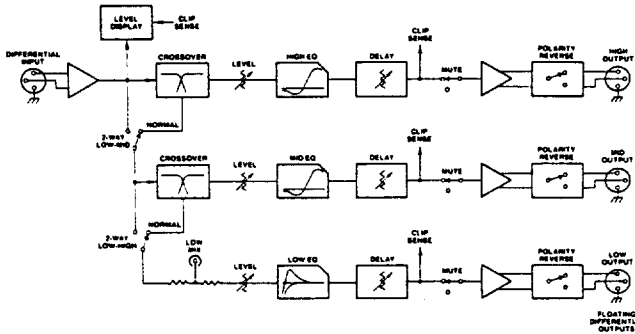
FIGURE 2 — XEQ-3 Crossover Block Diagram
