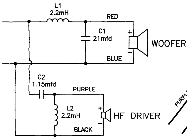
CROSSOVER SCHEMATIC
