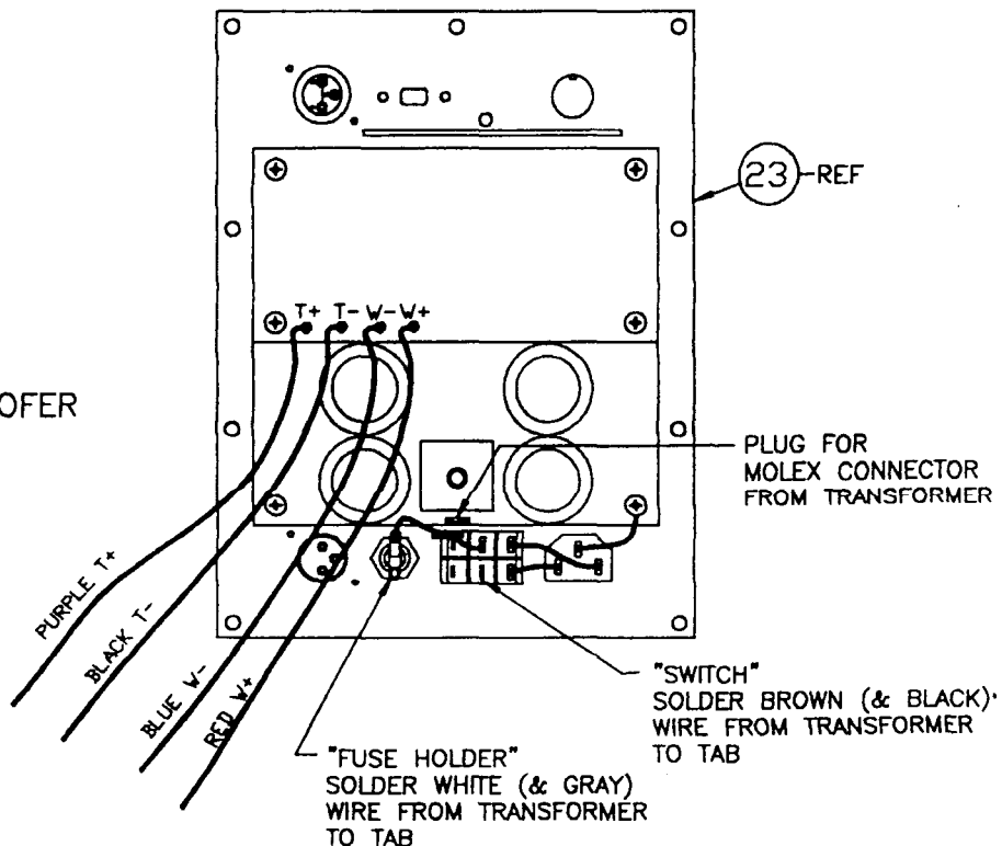
AMPLIFIER
