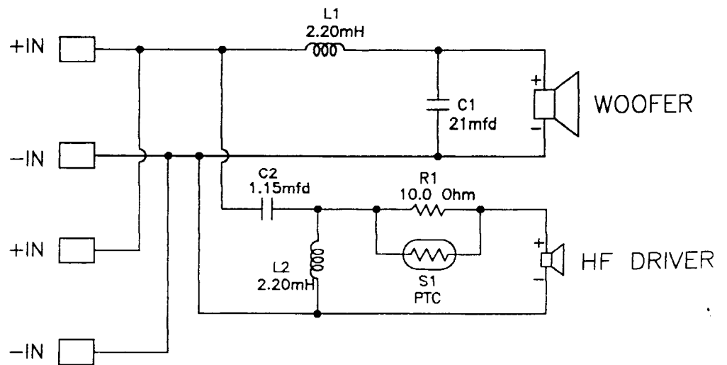
SCHMATIC DIAGRAM CROSSOVER P/N 84856 PRIOR TO DATE CODE 9906
