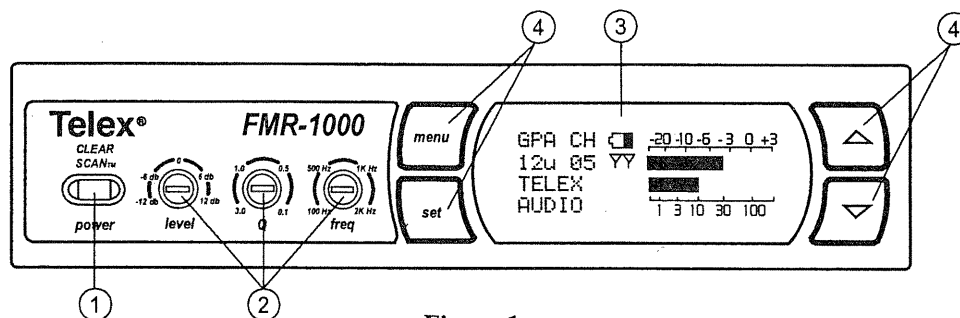
Figure 1 FMR-1000 Front Panel
