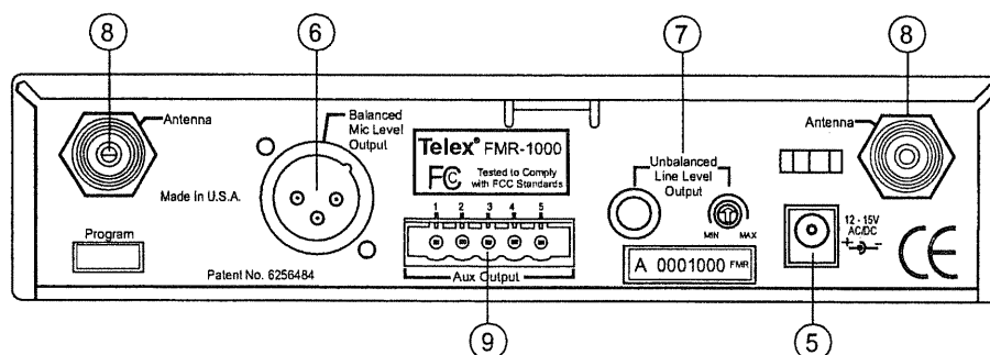
Figure 2 FMR-1000 Back Panel
