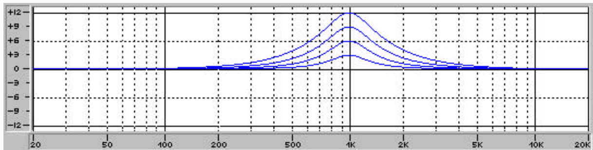
PEQ: f = 1kHz, Q = 2.0 Gain = +3dB, +6dB, +9dB, +12dB
