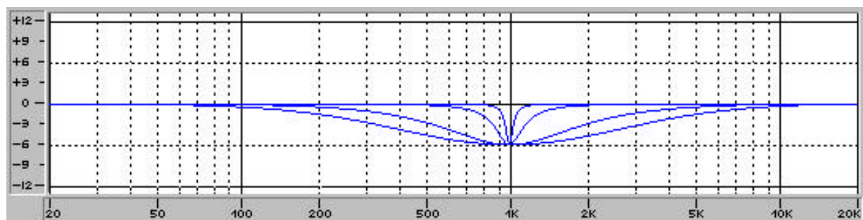
PEQ: f = 1kHz, Gain = -6dB Q = 0.5, 1.0, 5.0, 20.0
