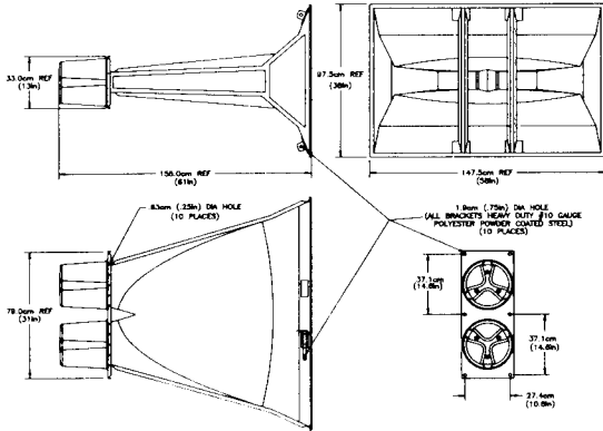
FIGURE 2 — Dimensions
