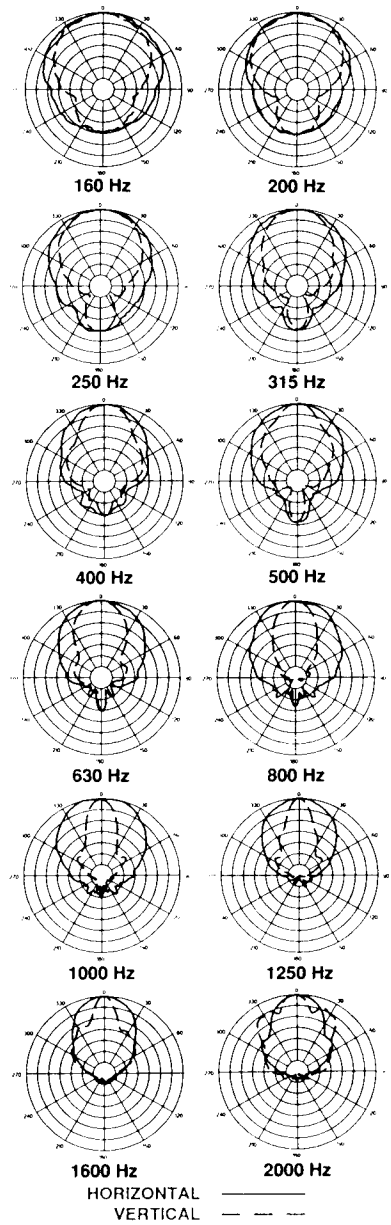
FIGURE 7 — Polar Response
