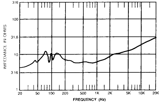
FIGURE 3 — Impedance Response
