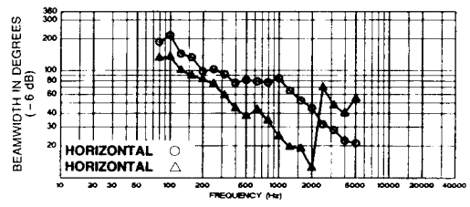
FIGURE 5 — Beamwidth Response
