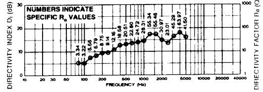
FIGURE 6 — Directivity Response
