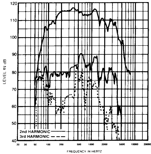
FIGURE 4 — Distortion Response, 10% Power
