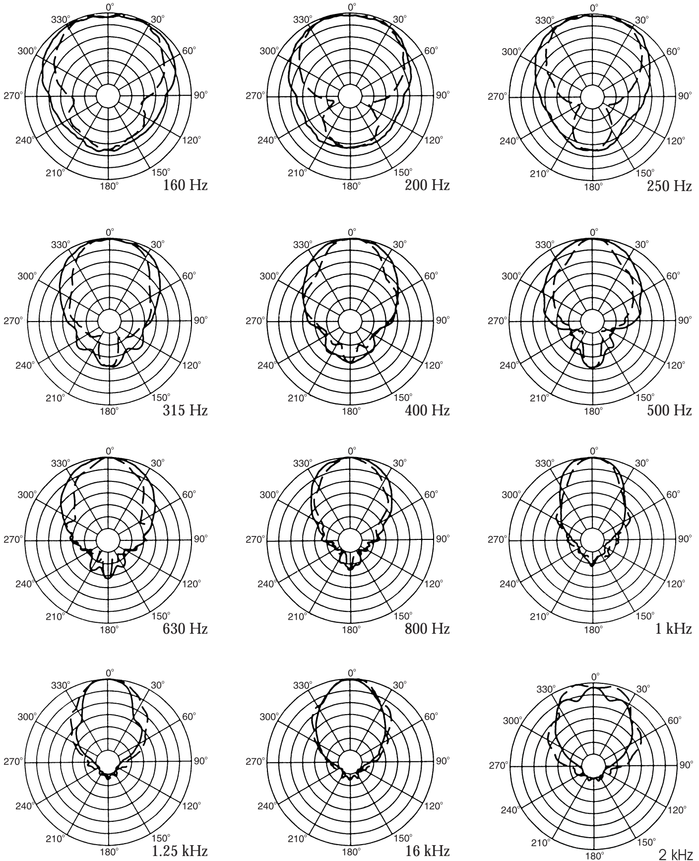
Figure 1—Polar Response
