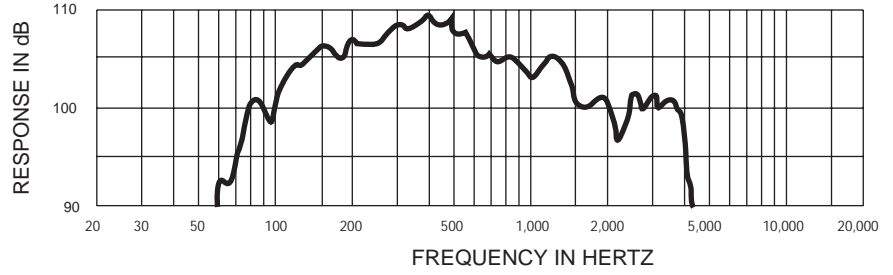
Figure 2—Axial Frequency Response (1 watt/1 meter)
