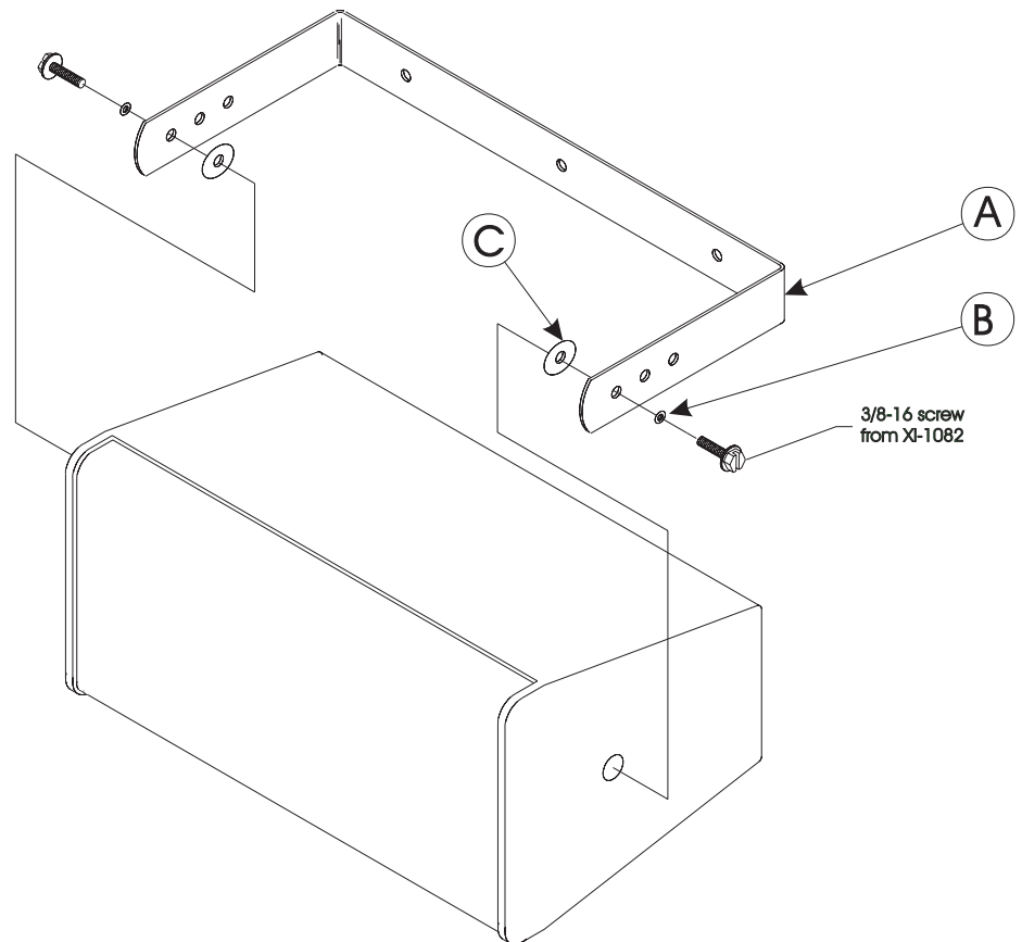
Figure 1 — Wall or Ceiling Mounting of Xi-1082 Speaker System with MB1082 Mounting Bracket
