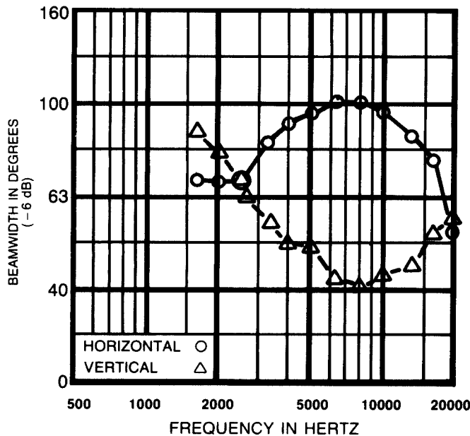
FIGURE 3 Beamwidth vs Frequency — HT94 Whole Space (Anechoic)
