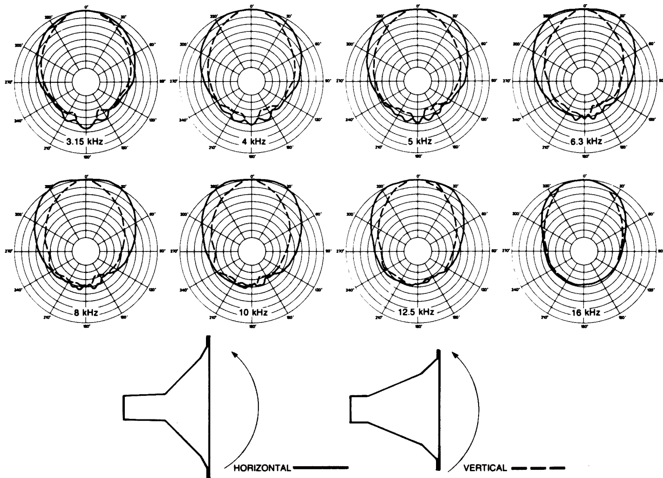
FIGURE 8 HT94 Polar Response (1/3 Octave Pink Noise, 4 Volts/10 Feet)
