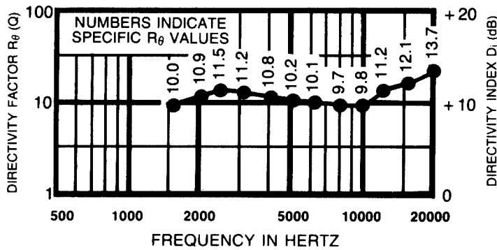
FIGURE 2 Directivity vs Frequency — HT94 Whole Space (Anechoic)
