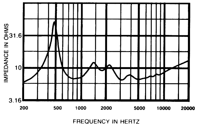
FIGURE 7 Impedance Response — DH1506 on HT94 Horn
