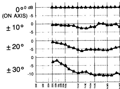
FIGURE 3 Vertical Off-Axis Response
