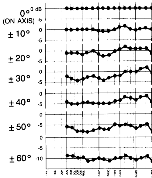
FIGURE 2 Horizontal Off-Axis Response
