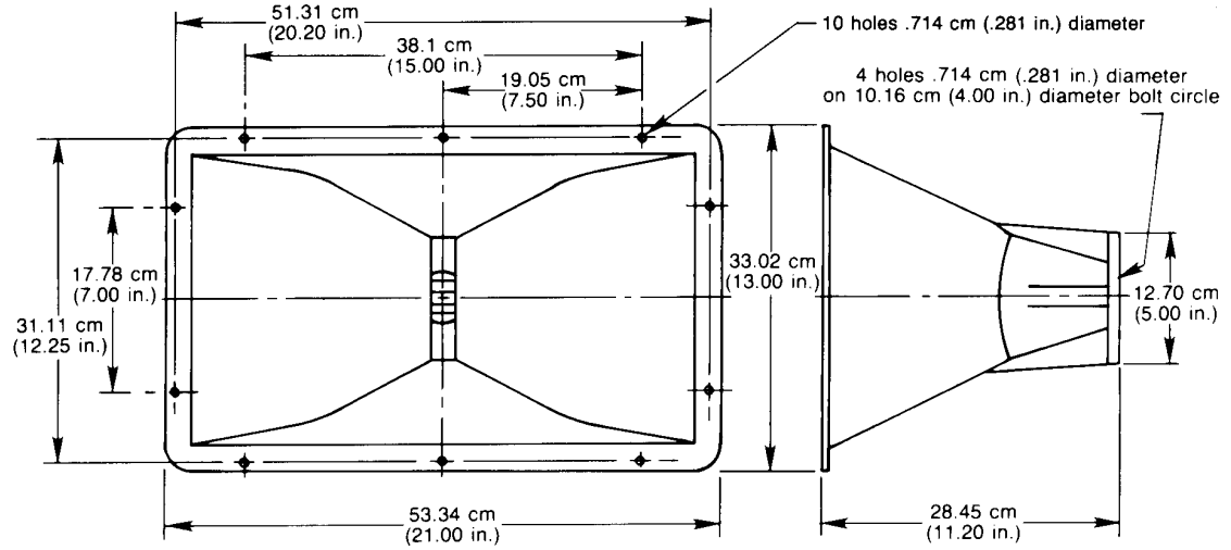
FIGURE 1 — Dimensions
