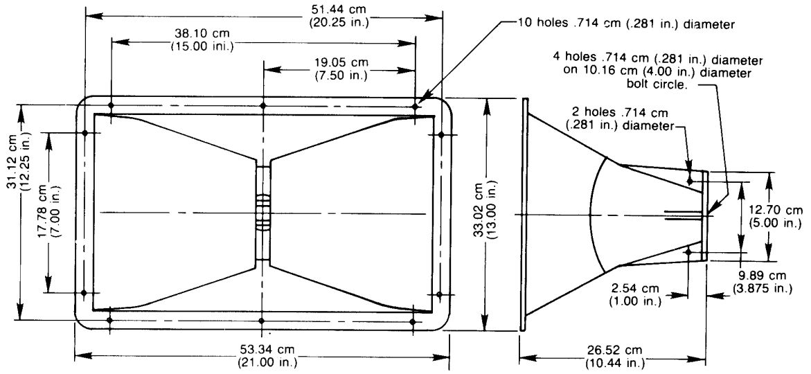
FIGURE 1 — Dimensions
