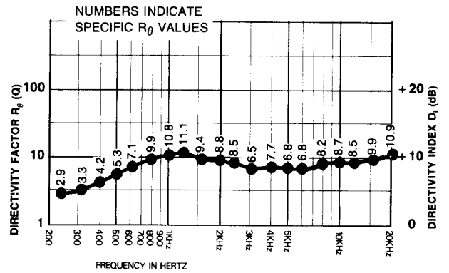
FIGURE 5 Directivity versus Frequency
