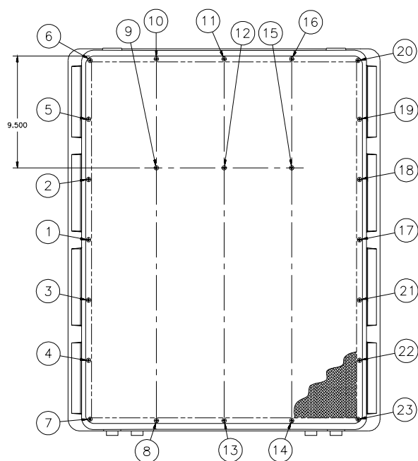
Figure 1—G500 installation order for attachment screws.
