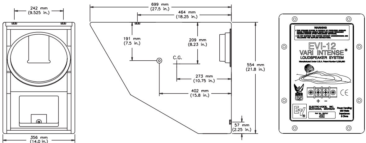
Figure 9—EVI-12 Dimensions
