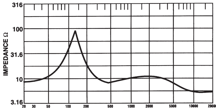
Impedance Response
