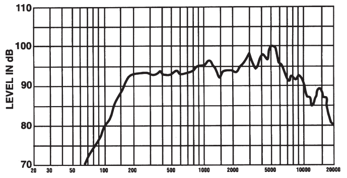
Frequency Response
