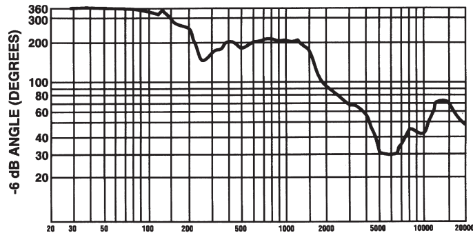
Beamwidth vs Frequency
