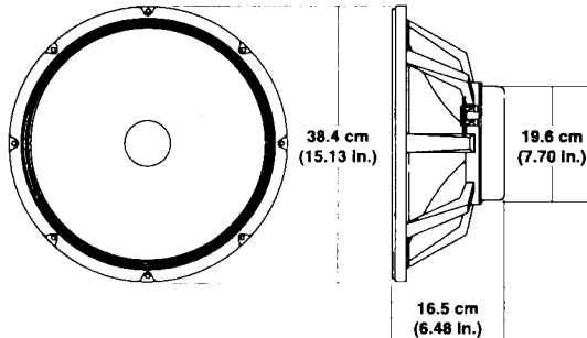
FIGURE 5 — Dimensions
