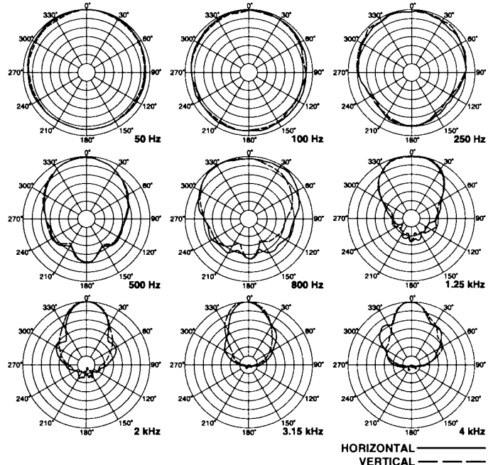
FIGURE 9 — Polar Response
