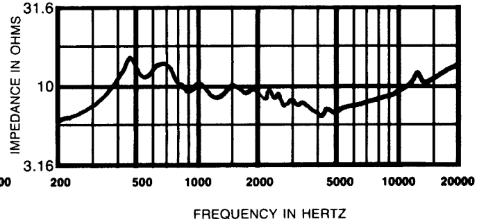
FIGURE 7 Impedance Response — HP64 Horn
