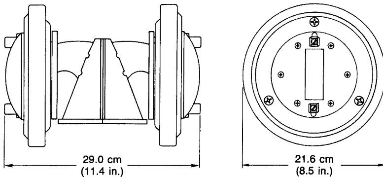
FIGURE 2 Dimensions
