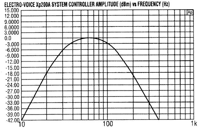
FIGURE 2 — Xp200A Frequency Response, Subwoofer Output, Profile Control Off (full counterclockwise)
