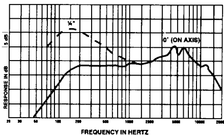
FIGURE 1 Frequency Response
