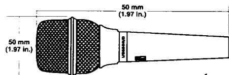
FIGURE 3 Dimensions
