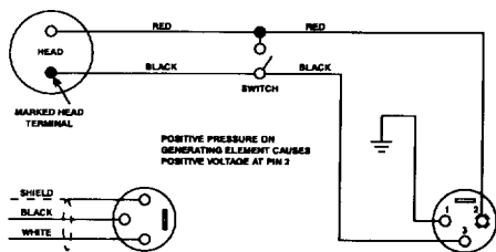
FIGURE 4 Wiring Diagram
