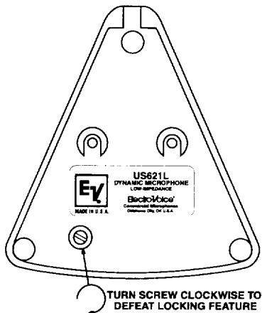
FIGURE 5 US621L/US622L Bottom View
