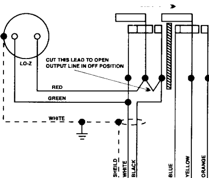
FIGURE 6 US621L/US622L Wiring Diagram
