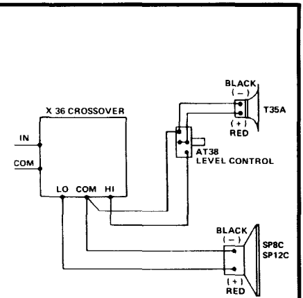
FIGURE 4 Two-Way System Wiring
