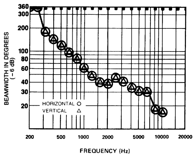
FIGURE 2 PH Beamwidth vs. Frequency
