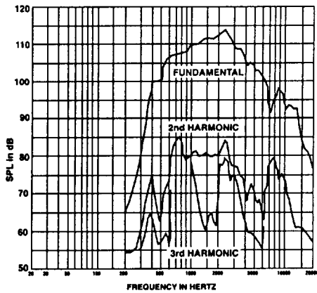
FIGURE 1 PA415 Frequency Response (1 watt at 1 meter)
