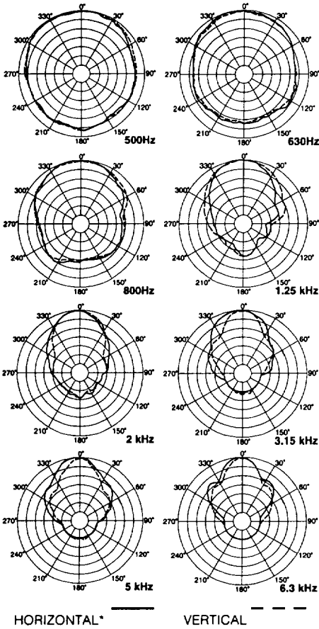
FIGURE 2 PA415 Polar Response
