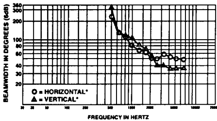
FIGURE 3 PA415 Beamwidth vs. Frequency
