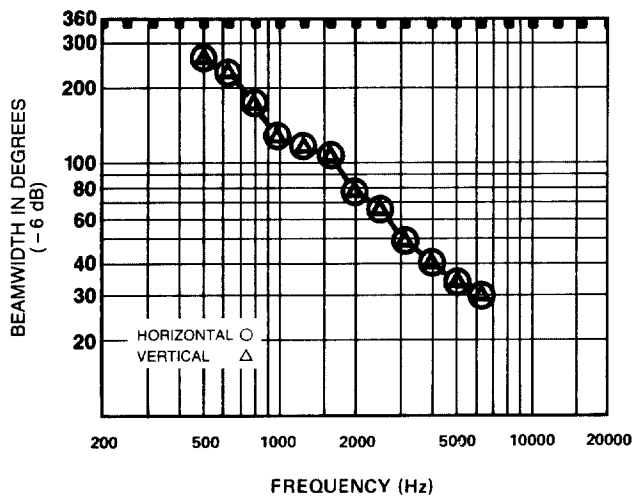
FIGURE 2 PA12 Beamwidth vs. Frequency
