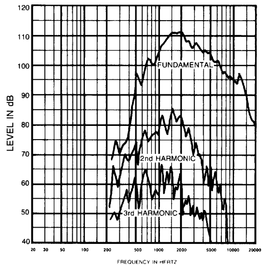
FIGURE 3 PA12 Frequency Response (1 watt at 1 meter)
