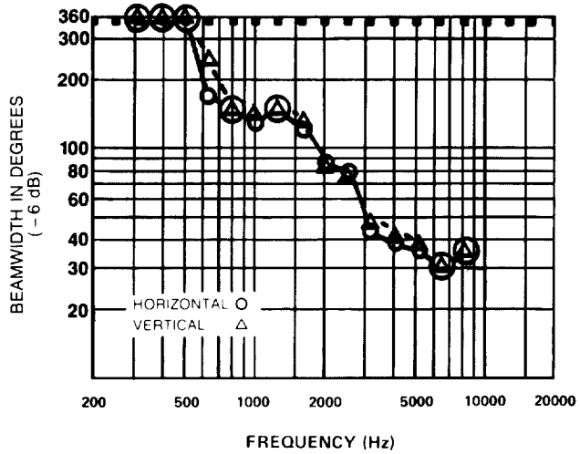
FIGURE 2 MM2TC Beamwidth vs. Frequency
