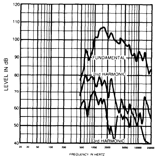
FIGURE 3 MIS4C/MIS8C Frequency Response (1 watt at 1 meter)
