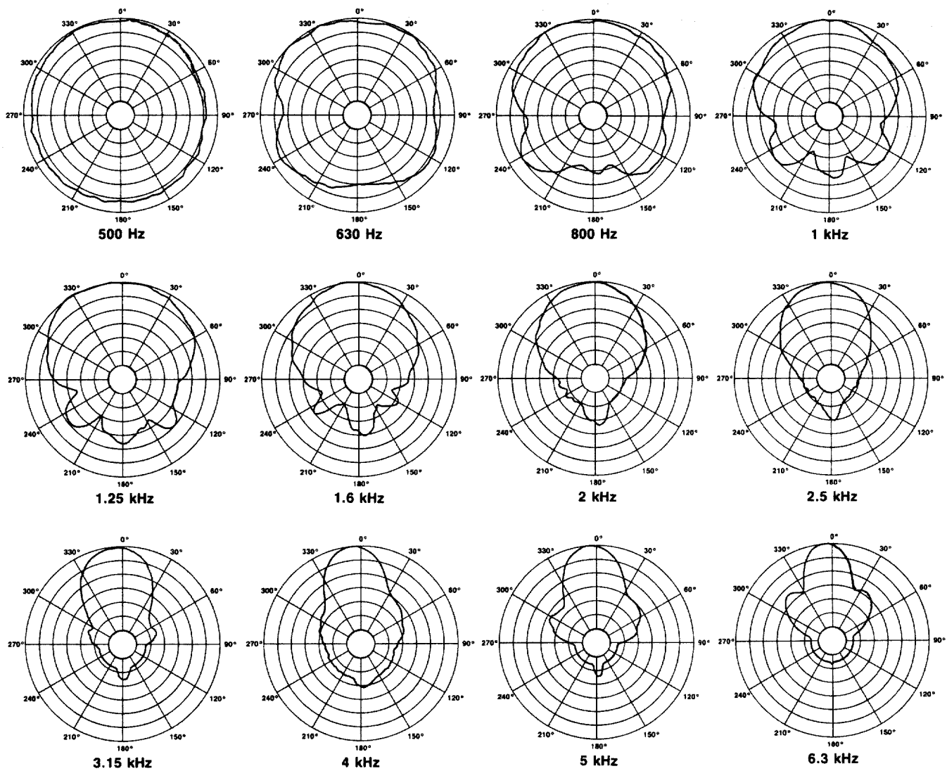
FIGURE 1 MILC Polar Response
