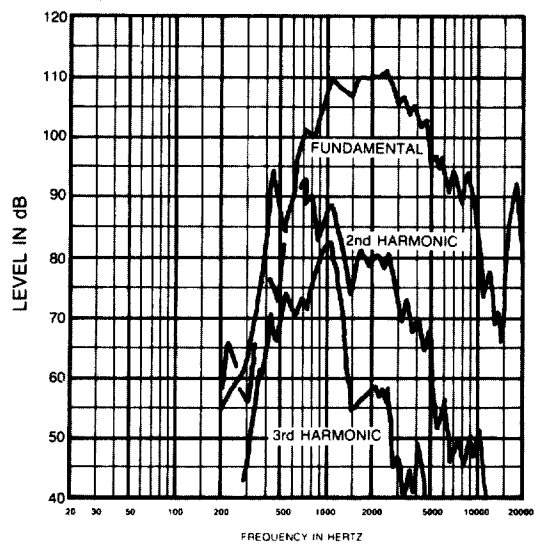
FIGURE 3 MILC Frequency Response (1 watt at 1 meter)
