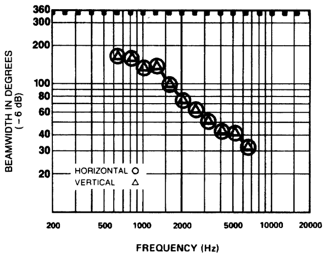
FIGURE 2 MILC Beamwidth vs. Frequency
