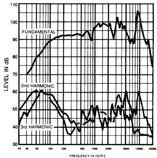
FIGURE 3 MC8A Frequency Response (1 watt at 1 meter)
