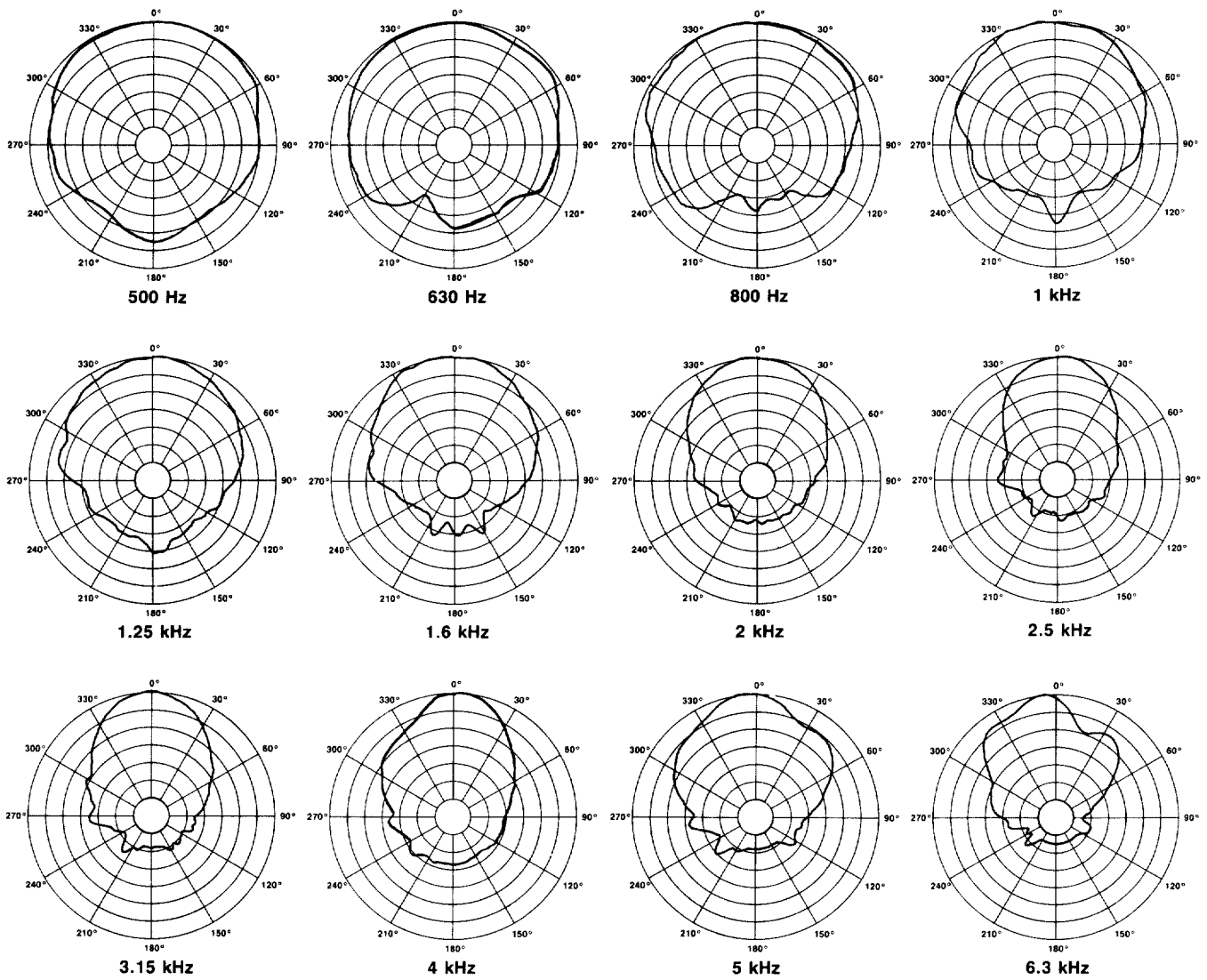
FIGURE 1 MC8A Polar Response
