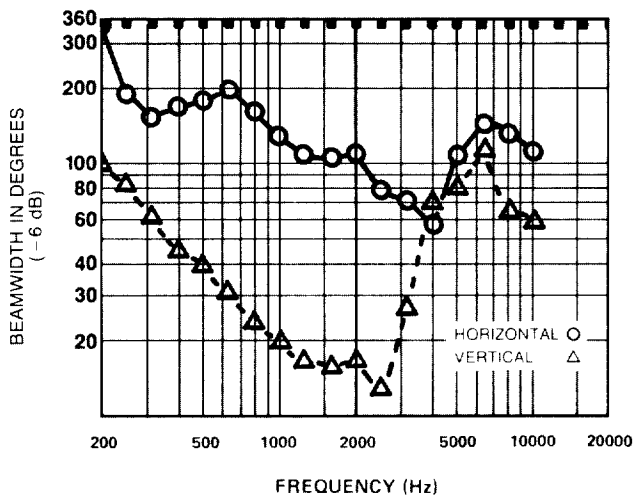
FIGURE 2 LR4B Beamwidth vs. Frequency
