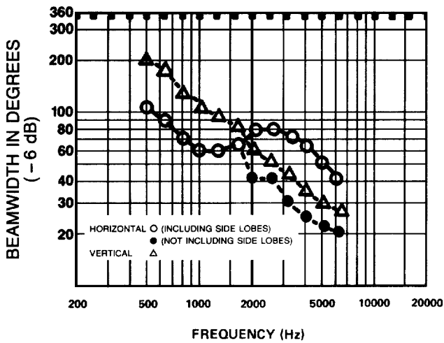
FIGURE 2 Cobreflex IIB Beamwidth vs. Frequency
