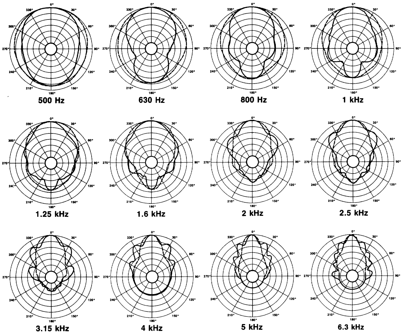
FIGURE 1 Cobreflex IIB Polar Response
