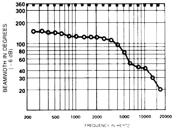
FIGURE 4 — CS410 Beamwidth vs. Frequency in 1.8 ft 3 Sealed Box
