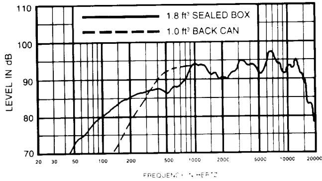
FIGURE 1 — Axial Frequency Response 1 Watt/1 Meter
