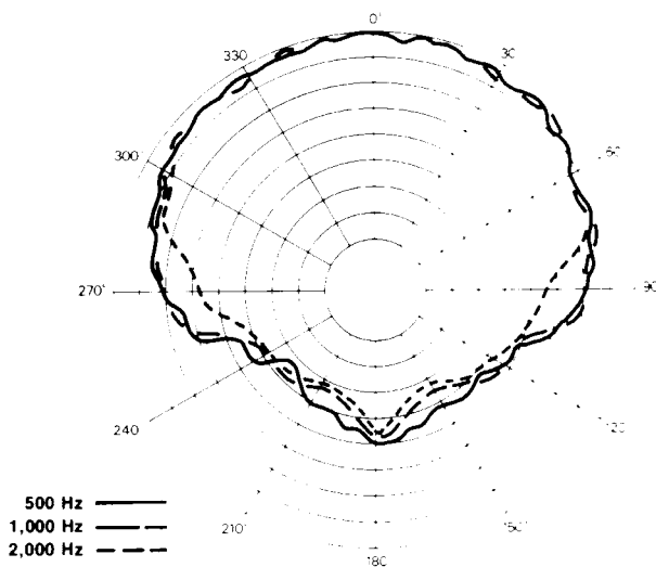
FIGURE 3 — CS410 Polar Response in 1.8 ft 3 Sealed Box 4V RMS of 1/3-Octave-Band-Limited Noise in Anechoic Environment, 10 Feet on Axis (5 dB per division)
