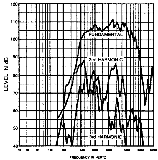
FIGURE 3 CFID15 Frequency Response (1 watt at 1 meter)
