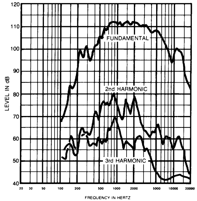
FIGURE 2 Distortion Response — FC100 Horn (1 watt at 1 meter)
