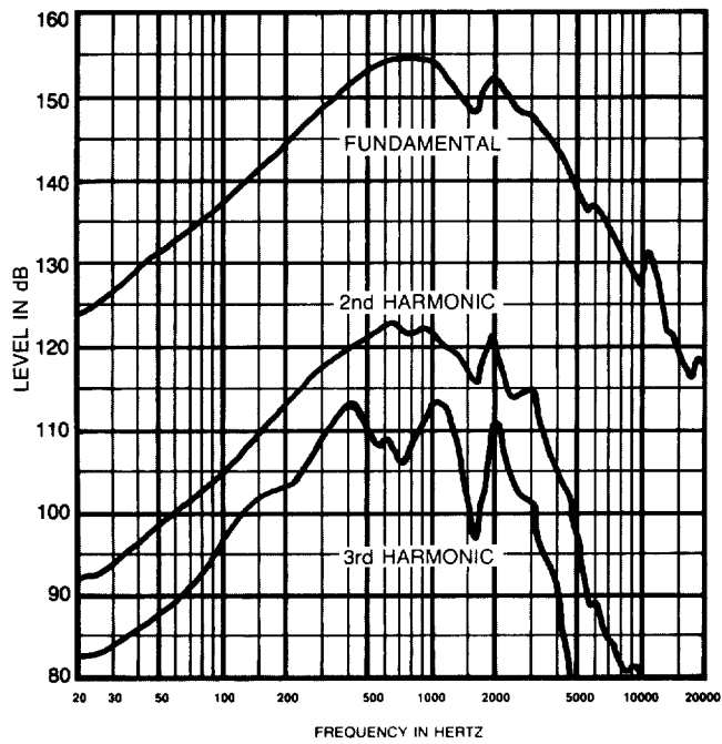
FIGURE 1 Distortion Response — Plane Wave Tube (1 inch) (4-watt input)
