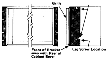
FIGURE 1 Bracket Locations for Rack Mounting Sentry® 100
