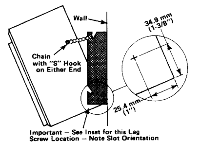
FIGURE 4 Angled Mount with System Vertical
