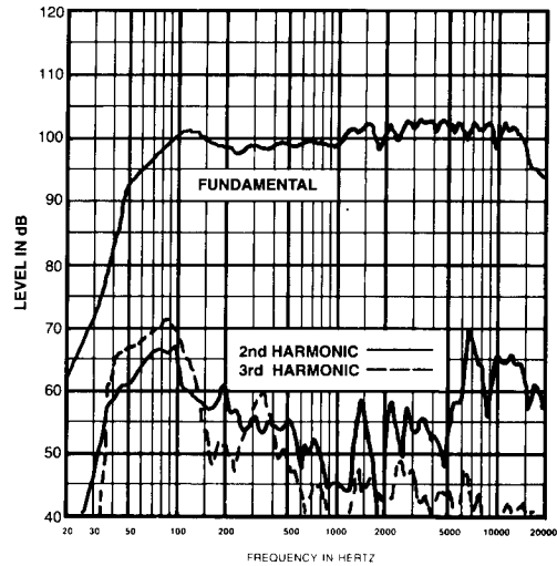
FIGURE 6 — Harmonic Distortion 0.1 Rated Power Input (10 watts)
