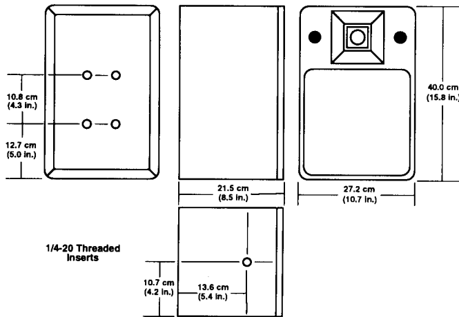
FIGURE 8 — Dimensions
