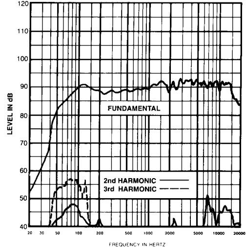
FIGURE 5 — Harmonic Distortion 0.01 Rated Power Input (1 watt)
