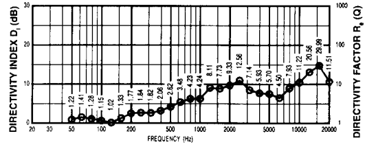
FIGURE 4 — Directivity vs. Frequency (whole space, anechoic environment)
