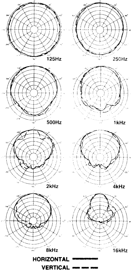
FIGURE 2 — Polar Response
