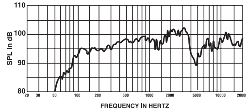
FIGURE 5 — PIM-102 Harmonic Distortion 10% Rated Input Power at 500 Hz (on axis at 1 meter from system)
