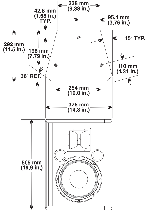
FIGURE 6 — PIM-102 Dimensions
