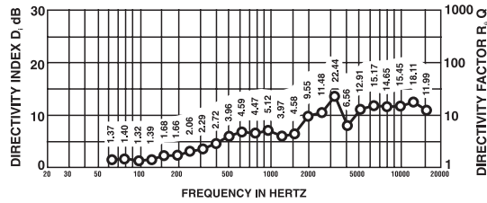
FIGURE 4 — PIM-102 Directivity Factor and Directivity Index vs. Frequency (one-third-octave bands of pink noise)
