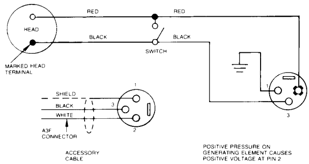
FIGURE 2 — Wiring Diagram
