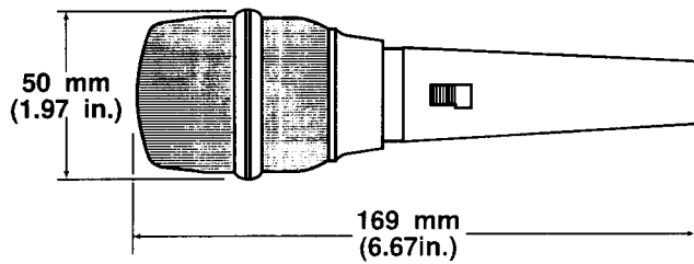
FIGURE 1 — Dimensions
