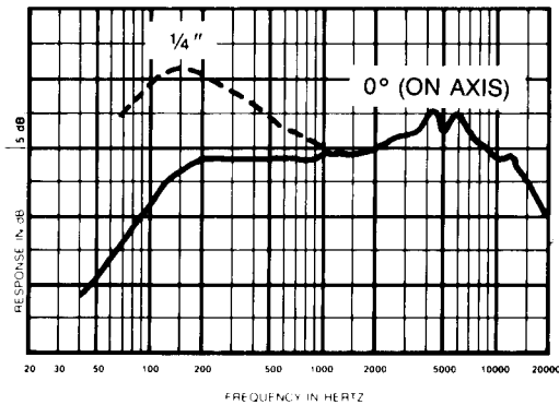
FIGURE 3 — Frequency Response
