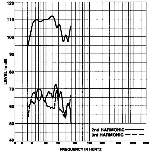
FIGURE 6 — Harmonic Distortion
