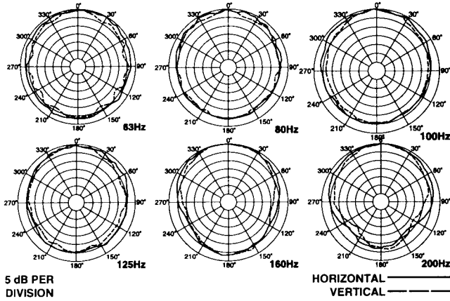
FIGURE 3 — Polar Response
