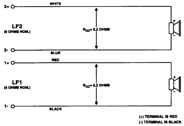
FIGURE 7 — Wiring Diagram
