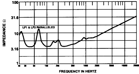
FIGURE 2 — Impedance vs. Frequency
