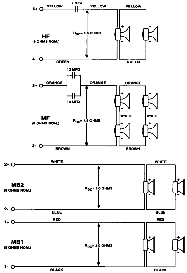
FIGURE 7 — MTH-4.5/64B Wiring Diagram
