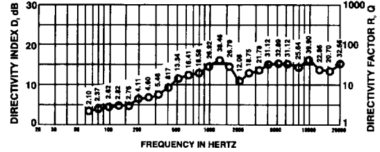
FIGURE 6 — MTH-4.5/64B Harmonic Distortion
