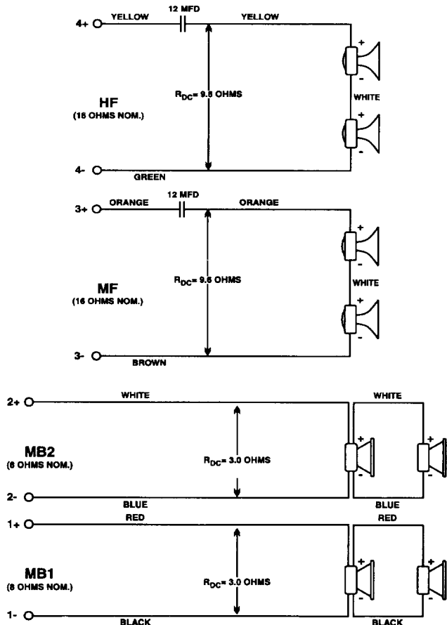
FIGURE 7 — Wiring Diagram
