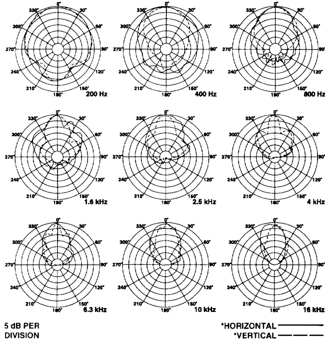
FIGURE 3 — Polar Response
