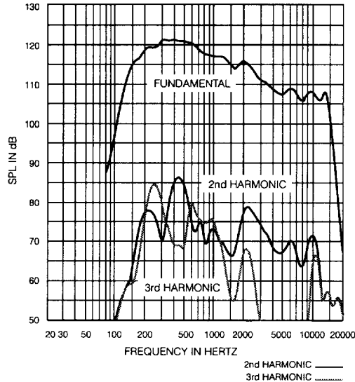
FIGURE 6 — Harmonic Distortion
