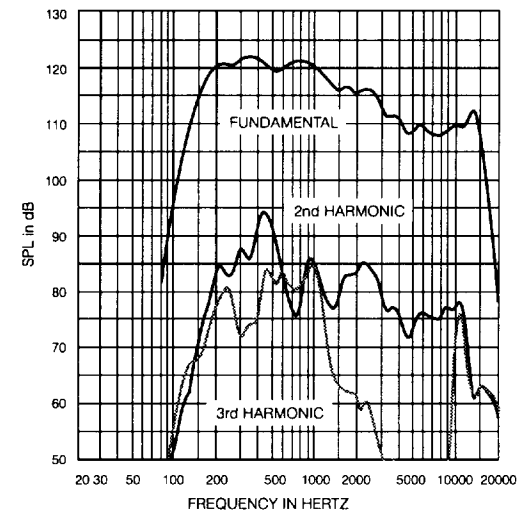
FIGURE 6 — MTH-2.5/64B Harmonic Distortion
