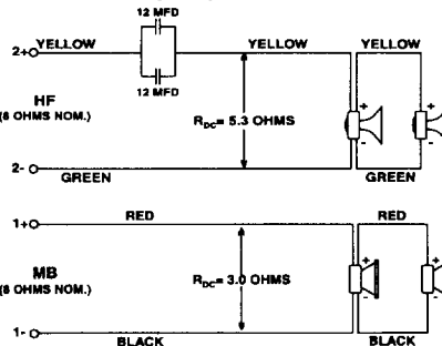
FIGURE 7 — MTH-2.5/64B Wiring Diagram
