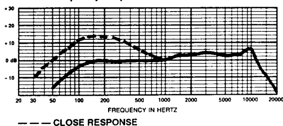
FIGURE 1 — Frequency Response
