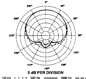
FIGURE 2 — Polars
