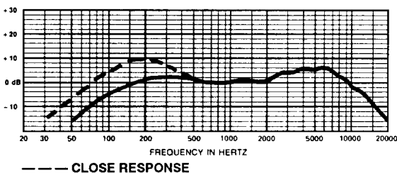
FIGURE 1 — Frequency Response
