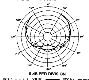
FIGURE 2 — Polars
