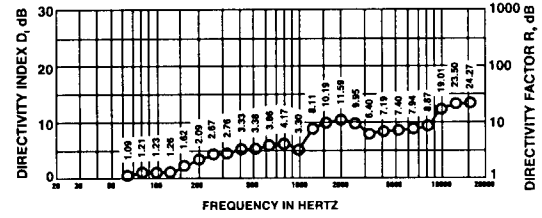
FIGURE 5 — Directivity vs. Frequency (anechoic environment)
