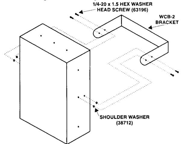
FIGURE 8 — Mounting the FR200B Using the WCB-2 Bracket
