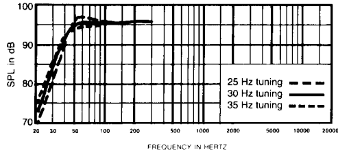
FIGURE 2A — EVX-180A Single-Driver Low-Frequency Performance: 170-Liter (6-ft³) Enclosure
