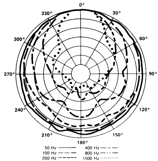
FIGURE 6 — Polar Response
