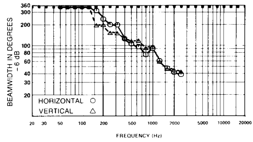
FIGURE 3 — Beamwidth vs. Frequency EVX-180A/TL3512 in a 255-Liter (9.0-ft³) Enclosure
