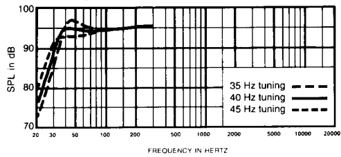
FIGURE 2C — EVX-180A Single-Driver Low-Frequency Performance: 283-Liter (10-ft³) Enclosure
