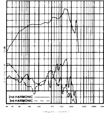
Distortion Response, 60 WATTS
