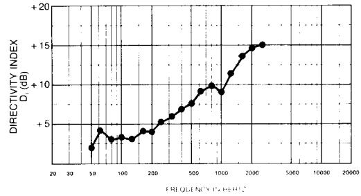
FIGURE 4 — Directivity Index vs. Frequency EVX-180A/TL3512 in a 255-Liter (9.0-ft³) Enclosure
