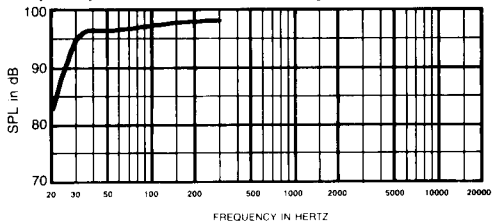
FIGURE 2D — EVX-180A Multiple-Driver Low-Frequency Performance: Two Drivers In a 566-Liter (20-ft³) Box or Two 283-Liter (10-ft³) Boxes in Close Proximity Tuned to 30 Hz
