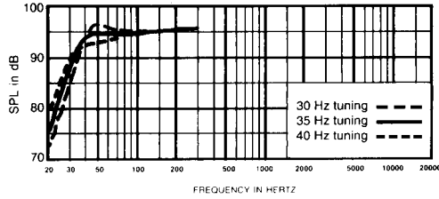
FIGURE 2B — EVX-180A Single-Driver Low-Frequency Performance: 227-Liter (8-ft³) Enclosure
