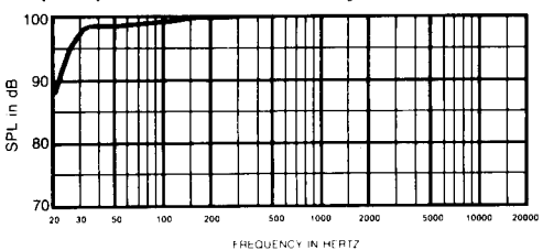
FIGURE 2E — EVX-180A Multiple-Driver Low-Frequency Performance: Four Drivers In a 1,132-Liter (40-ft³) Box or Four 566-Liter (20-ft³) Boxes in Close Proximity Tuned to 28 Hz
