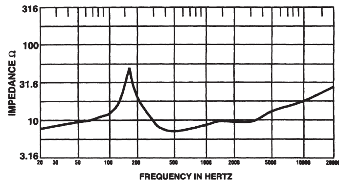
Impedance Response
