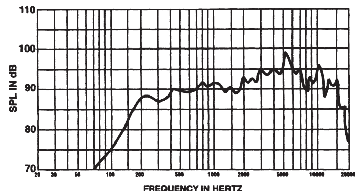
Frequency Response
