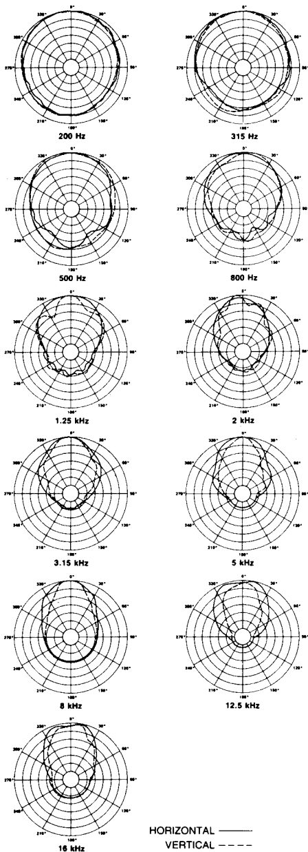
FIGURE 2 — DML-1152A/DMC-1152A Polar Response (1/3-octave pink noise, 4 volts at 20 feet)
