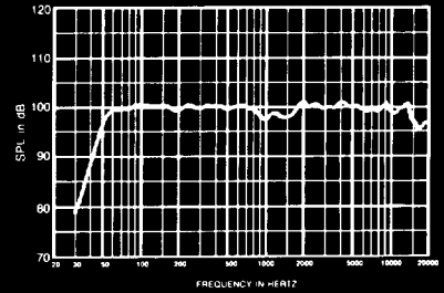
FIGURE 1 — DML-1152A/DMC-1152A Axial Frequency Response (1 watt/1 meter into LF midband)
