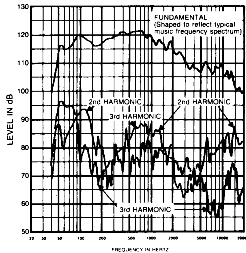
FIGURE 5 — DML-1152A/DMC-1152A Harmonic Distortion (120 dB SPL/1 meter using typical music frequency spectrum)
