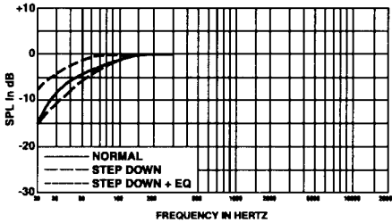
FIGURE 11 — Maximum SPL at 1 Meter in Typical Enclosure (8.0 ft 3 tuned to 45 Hz)
