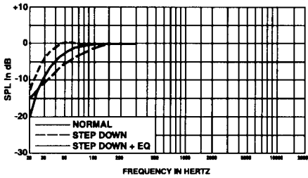
FIGURE 10B — Predicted Low-Frequency Response in a Typical Enclosure (12.0 ft 3 tuned to 25 Hz)
