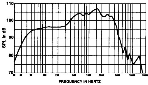
FIGURE 1 — Axial Response in Typical Enclosure (8.0 ft 3 ), 1 Watt/1 Meter
